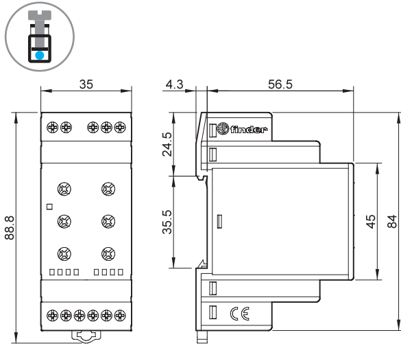
Type 70.61 Screw terminal
