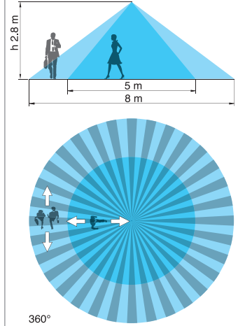
18.01, 18.11 - Ceiling mounting
