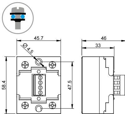
Type 77.x2 Screw terminal (plate clamp)
