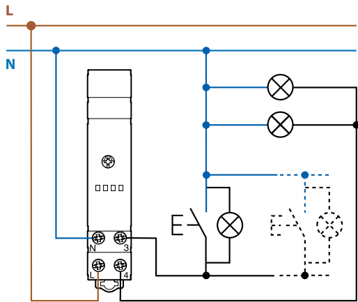
3 wire connection
