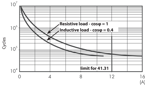
F 41 - Electrical life (AC) v contact current (bistable)
