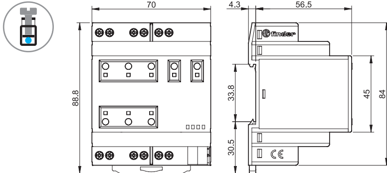
Type 19.3K/ 19.6K Screw terminal
