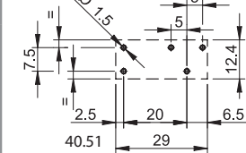
Copper side view
