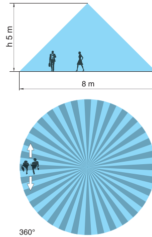
18.31.8.230.0000/18.21.8.230.0000 - Ceiling mounting
