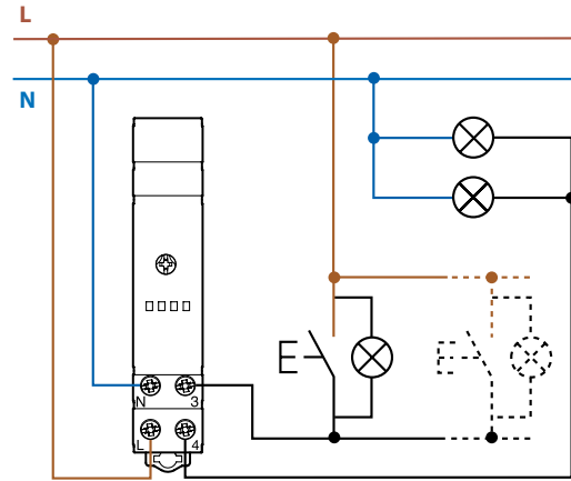
4 wire connection
