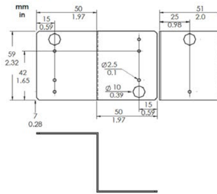
VYX 001 Surface Mounting Plate for sensors
