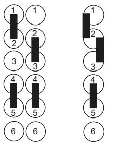
Mechanical Interlock (XACA009)
