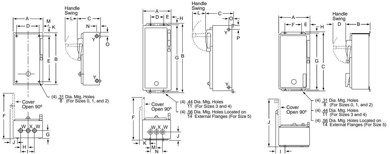
Figure 16.15: NEMA 1 Enclosure (Sizes 0–2) Figure 16.16: NEMA 1 Enclosure (Sizes 3–6) Figure 16.17: NEMA 12/3R Enclosure
