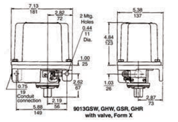
9013GSW, GHW, GSR, GHR with valve, Form X
