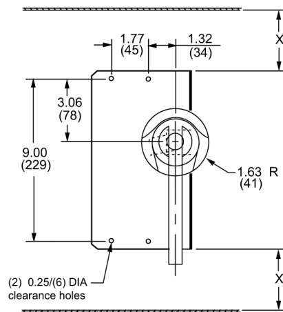
Panel Drilling for PowerPac™ D and L Circuit Breaker Operating Mechanisms: 9421LD1, 9421LD4, and 9421LD7 W/standard 6-inch handle
