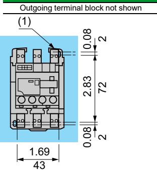
Panel mounting
